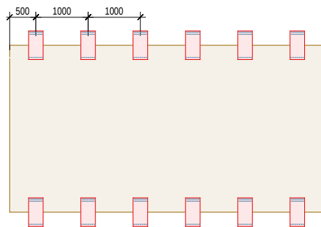
Figure 12: Wall element with position of slotted plates (source: Assmann)
