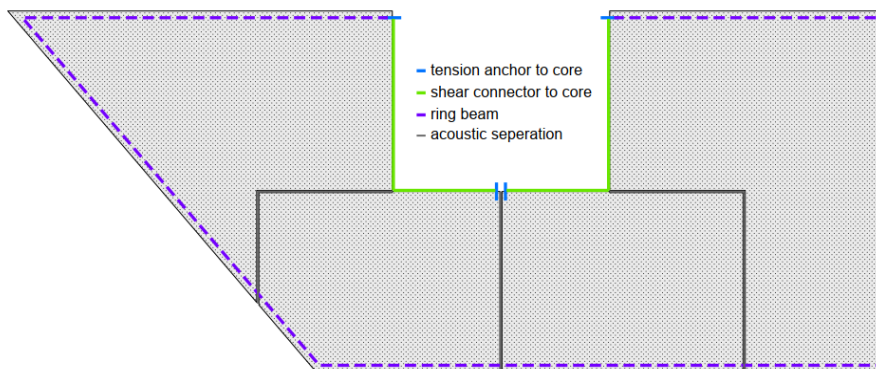
Figure 8: Diaphragm principle (source: RWT plus)
