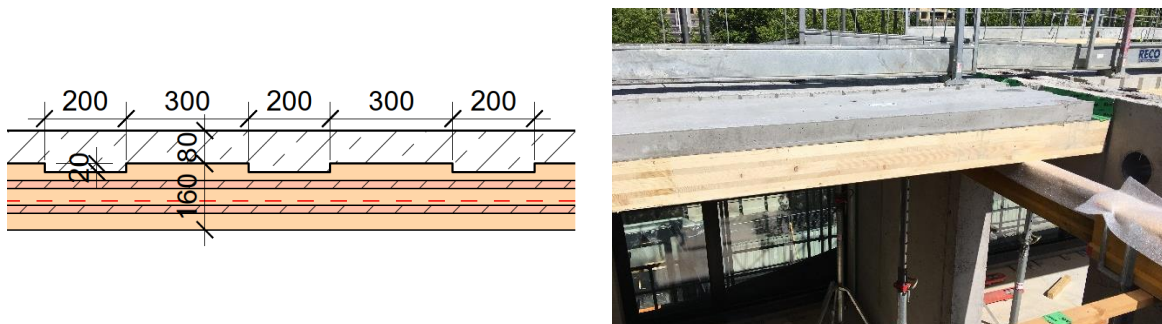
Figure 7: Floor build-up
