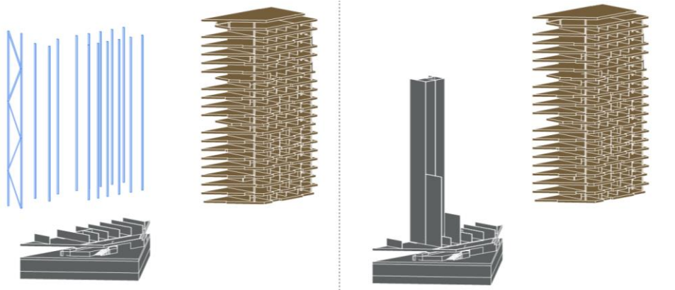
Figure 5: Stability system, steel-timber hybrid (left) and concrete-timber hybrid (right)
