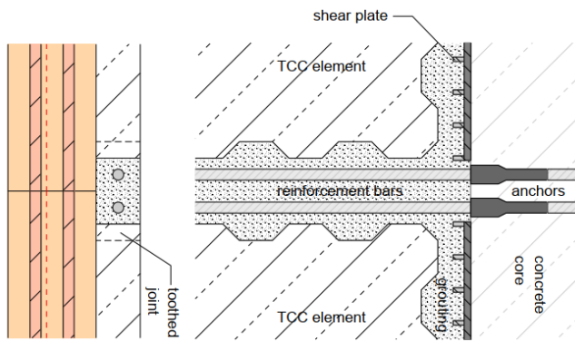
Figure 9: Joint between TCC-elements and core (source: RWT plus)
