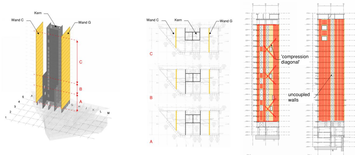
Figure 6: Lateral force resisting system (left) and elevation of CLT shear walls
